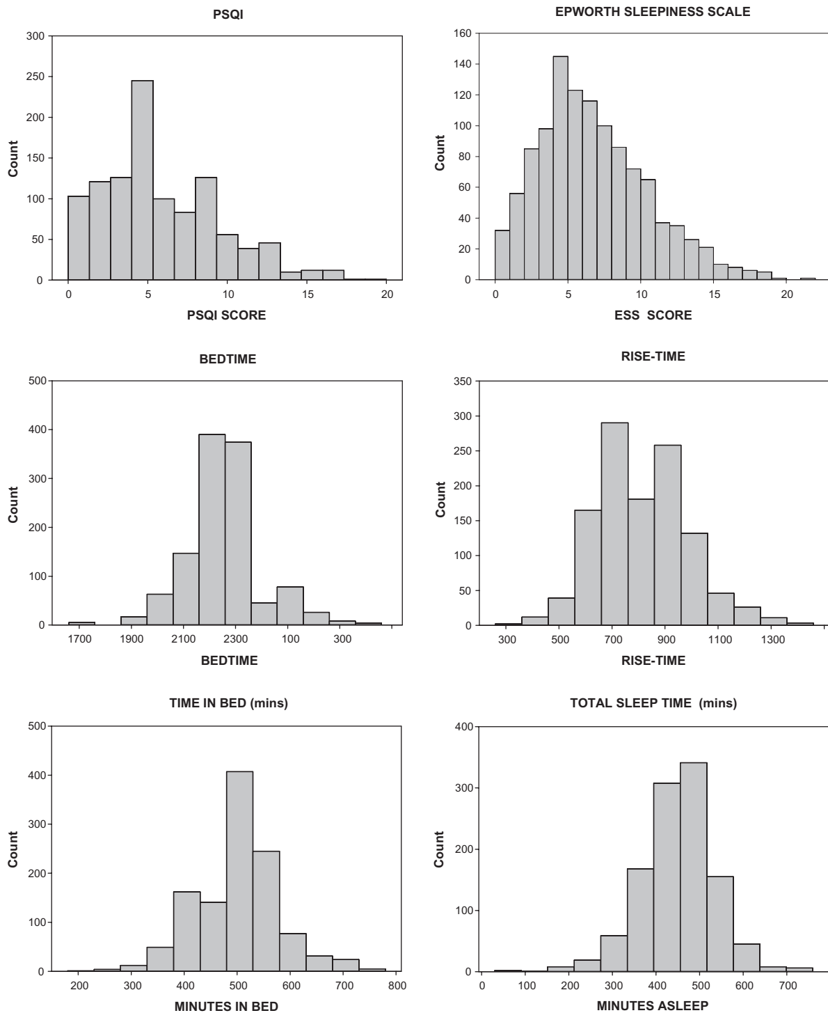
Figure 1. Frequency histograms for each of the six variables.
