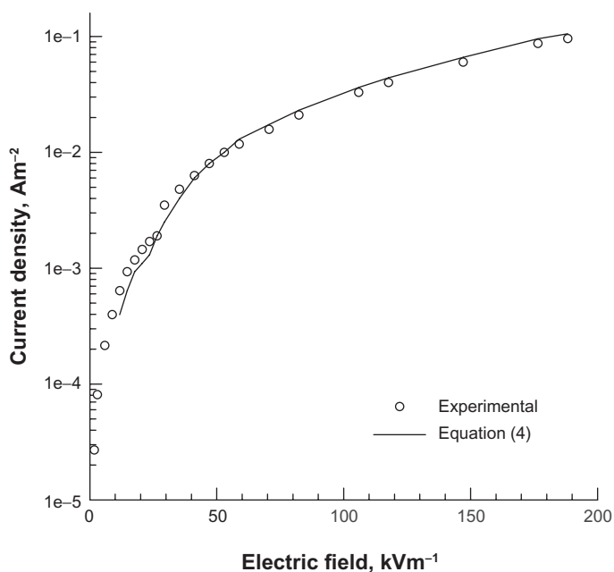
Figure 2. Log current density for S5 30/0 versus electric field at room temperature: experimental data and fitting using Eq. (4).
