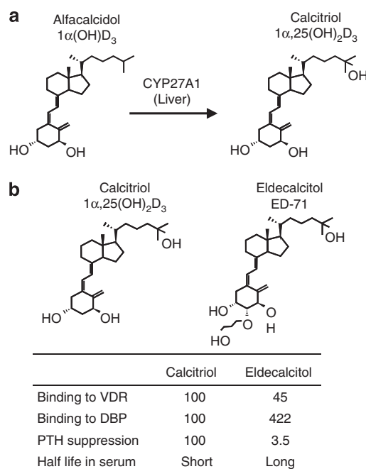
Figure 7 Structures and characteristics of vitamin D compounds used as therapeutic drugs for osteoporosis. (a) Alfalcidol, a prodrug of calcitriol (1 \alpha ,25(OH) 2 D 3 ), is metabolized to calcitriol by liver CYP27A1. Alfalcidol, therefore, acts as calcitriol in vivo . (b) Eldecalcitol has a hydroxypropoxy substituent at the 2 \beta position. Eldecalcitol is not metabolized to calcitriol in vivo . Some characteristics of eldecalcitol are compared with those of calcitriol.
