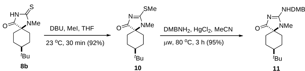
Scheme 3. Guanidinylation of 2-thiohydantoin 8b
