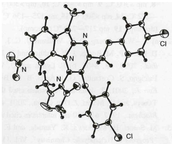
Figure 4. ORTEP Drawing of 18 (R = 0.045)
