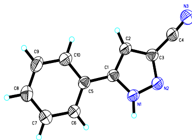
Figure 1. ORTEP diagram of 2c with the atomic labeling scheme
