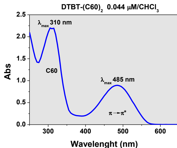
Figure 1. DTBT-(C 60 ) 2 absorption UV-Vis spectrum of a 0.044 μM solution in CHCl 3
