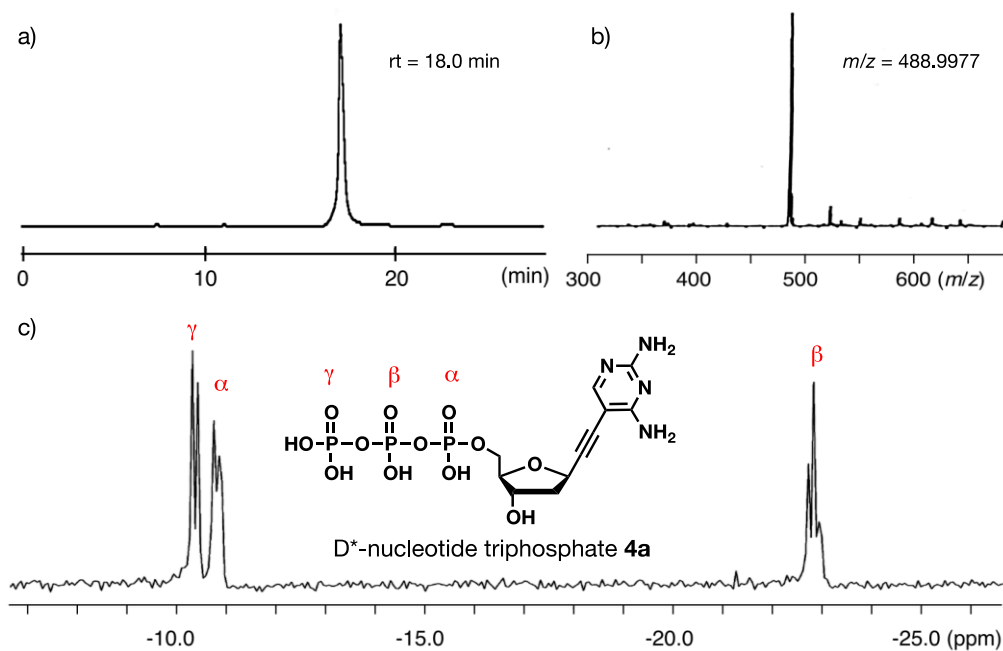
Figure 1. (a) A reverse-phase HPLC profile of D*-nucleotide triphosphate 4a after purification (5C 18 -AR-II column: 100 mM triethylammonium acetate (pH 7.0)/MeCN, 0 → 40%, 90 min). (b) ESI-HRMS spectrum of 4a under a negative ion mode (calcd for [M-H] - , C 11 H 16 N 4 O 12 P 3 : 488.9983). (c) 31 P NMR (160 MHz) spectrum of 4a in D 2 O at room temperature.
