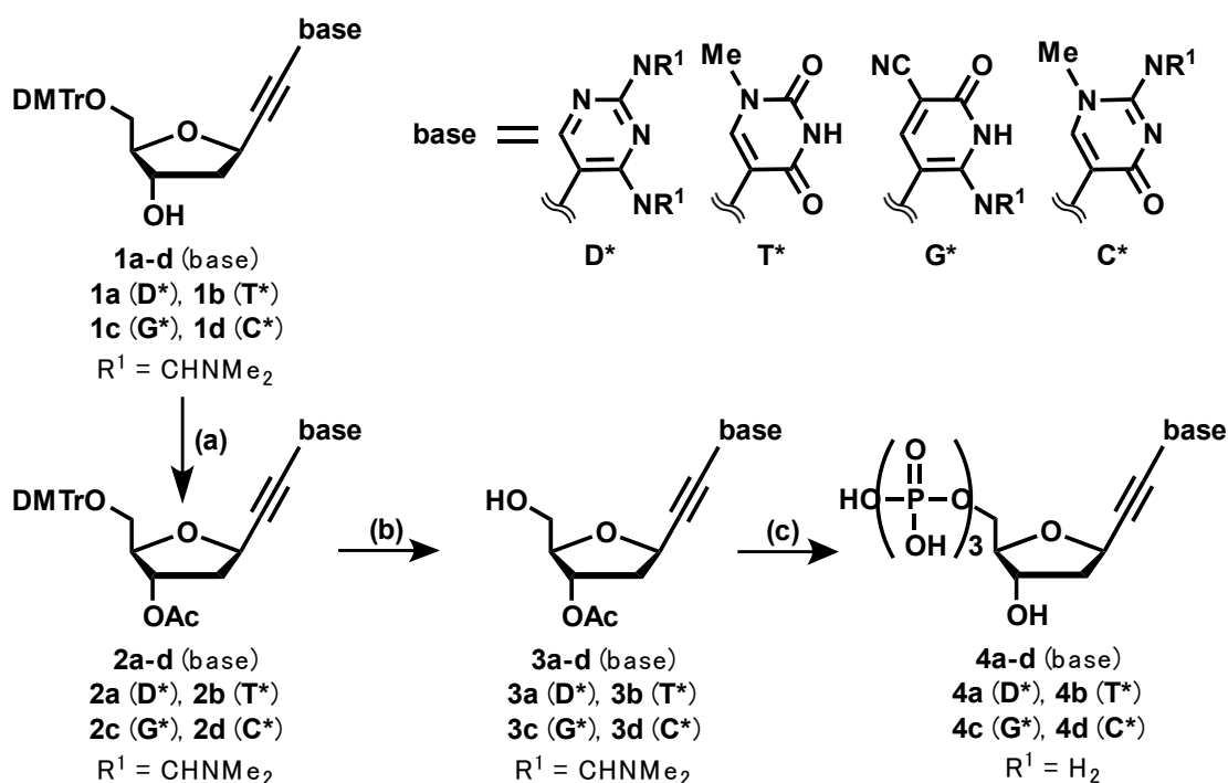
Scheme 1. (a) \text{Ac}_2\text{O} , DMAP, \text{Et}_3\text{N} , pyridine; (b) \text{CCl}_3\text{CO}_2\text{H} , pyridine, \text{CH}_2\text{Cl}_2 , (59% for 3a , 69% for 3b , 90% for 3c , 52% for 3d , in 2 steps); (c) 1) 2-chloro-4 H -1,3,2-benzodioxaphosphorin-4-one, pyridine, MeCN, 2) bis(tri- n -butylammonium)pyrophosphate, tributylamine, DMF, 3) iodine (1%) in pyridine- \text{H}_2\text{O} , 4) \text{NH}_4\text{OH} , \text{H}_2\text{O} , (3% for 4a , 28% for 4b , 2% for 4c , 4% for 4d ).
