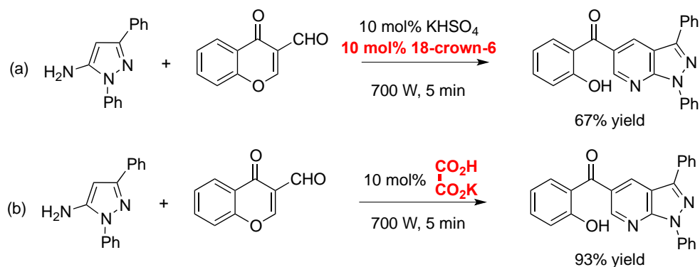
Scheme 3. Control experiments
