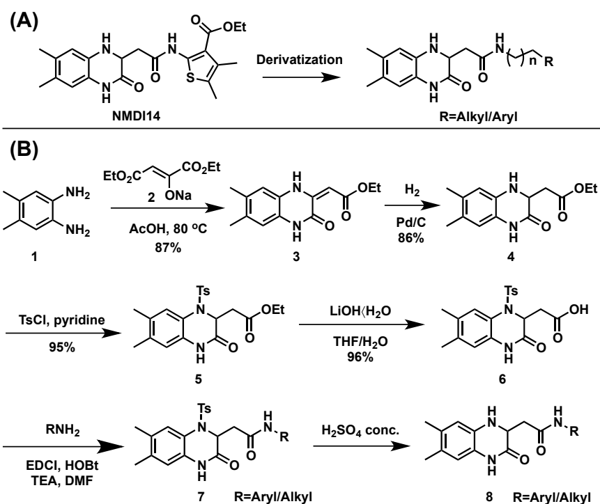
Figure 3. (A) Derivatization of NMDI14 at amide side chains. (B) Synthetic schemes for NMDI14 derivatives.
