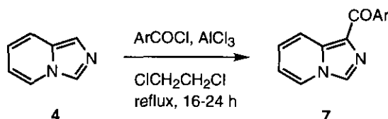
Scheme 2. Friedel-Crafts Acylation at the C1-Position of Imidazo[1,5- a ]pyridine.
