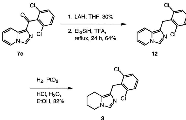
Scheme 5. Synthesis of Target Analogs (12) and (3).
