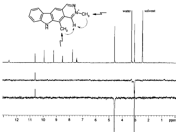
Figure 1. 300 MHz 1 H-NMR spectrum (upper trace) and NOE difference spectra of 14 (DMSO-d 6 , 28°C), with the resonances of CH 3 -5 (3.09 ppm; middle trace) and CH 3 -3 (4.61 ppm; lower trace) as irradiation points.
