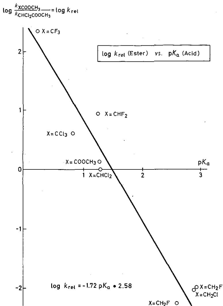
Figure 3. Correlation between the \log k_{\text{rel}} of the addition reactions of benzonitrilio-2-propanide ( 3e ) to methyl-esters and the \text{pK}_{\text{a}} 's of the acids of the corresponding methyl esters.
