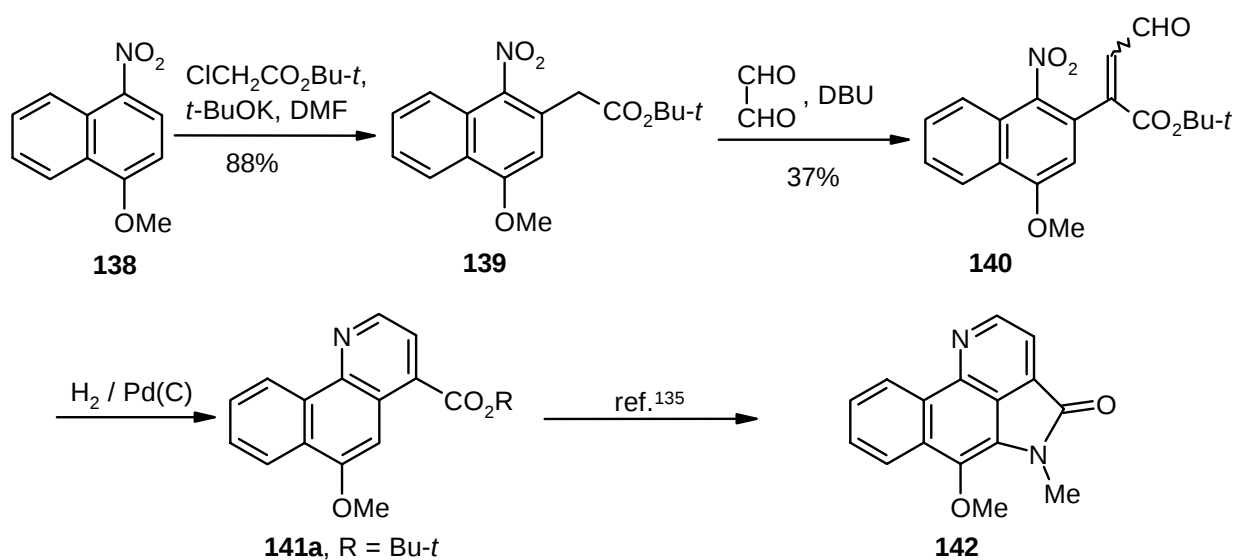
Scheme 36
