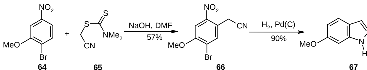
Scheme 18
