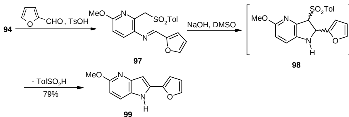
Scheme 27
