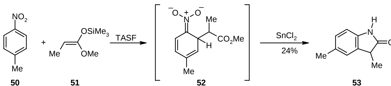
Scheme 15
