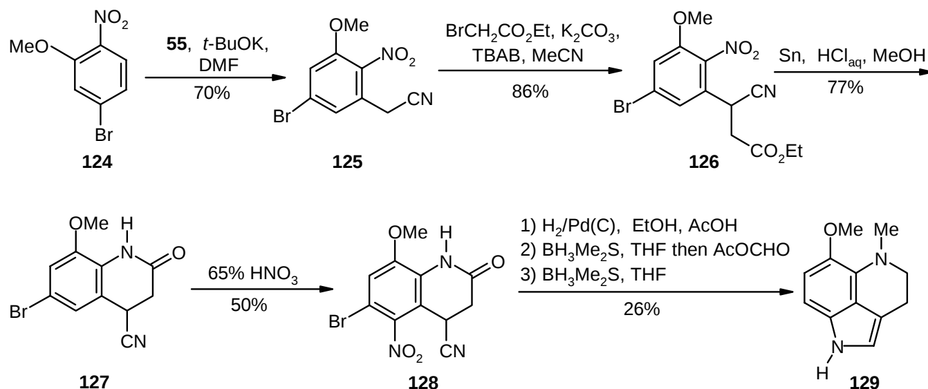
Scheme 34
