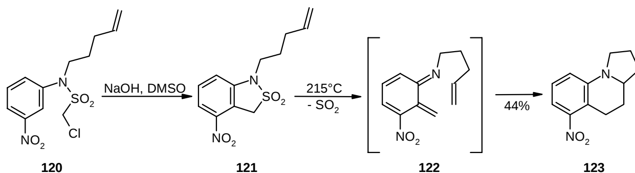
Scheme 33
