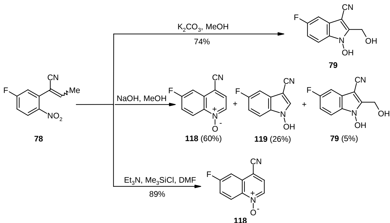
Scheme 32
