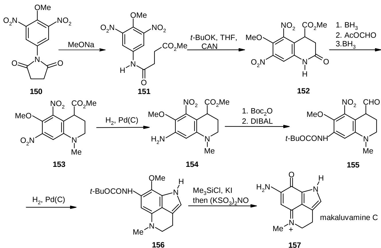
Scheme 39
