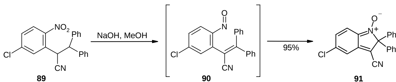
Scheme 25
