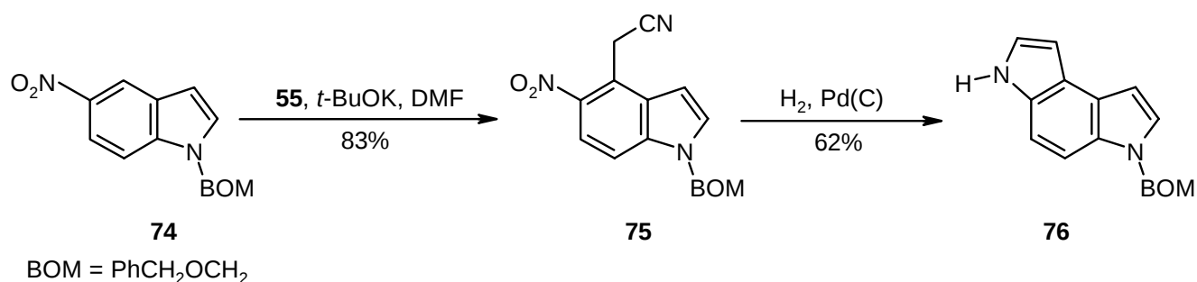
Scheme 21
