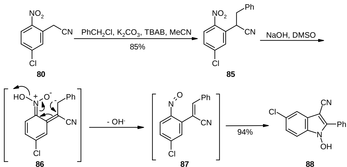
Scheme 24
