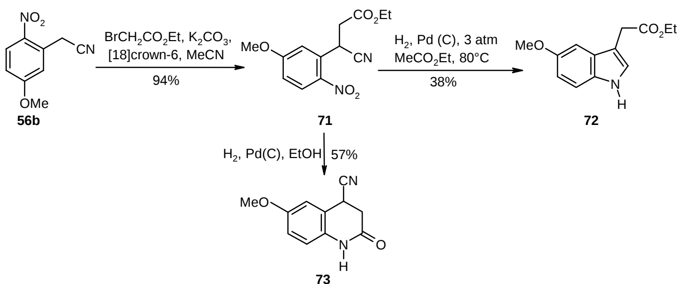
Scheme 20
