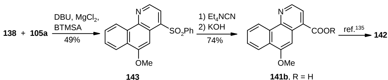
Scheme 37
