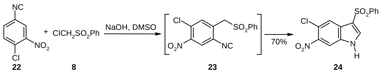
Scheme 7
