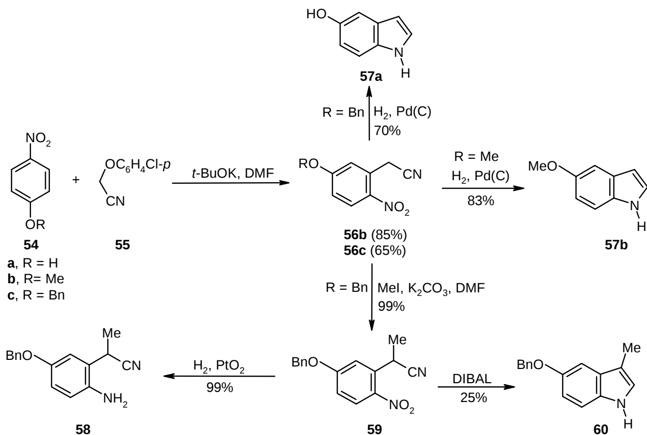
Scheme 16
