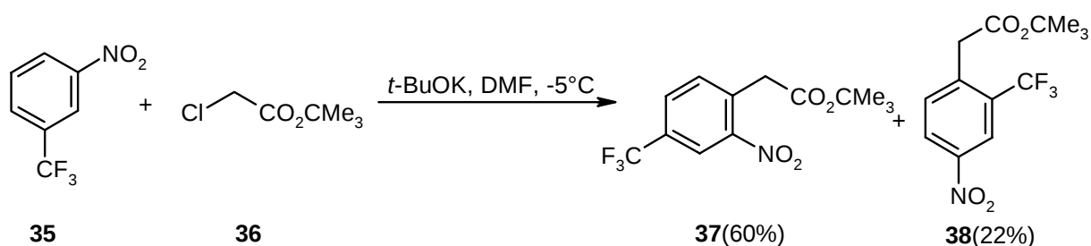
Scheme 11.
