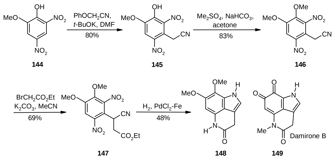
Scheme 38
