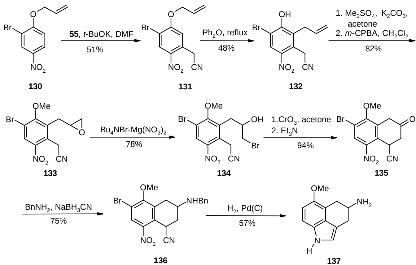
Scheme 35
