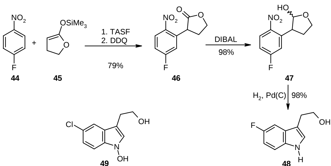
Scheme 14
