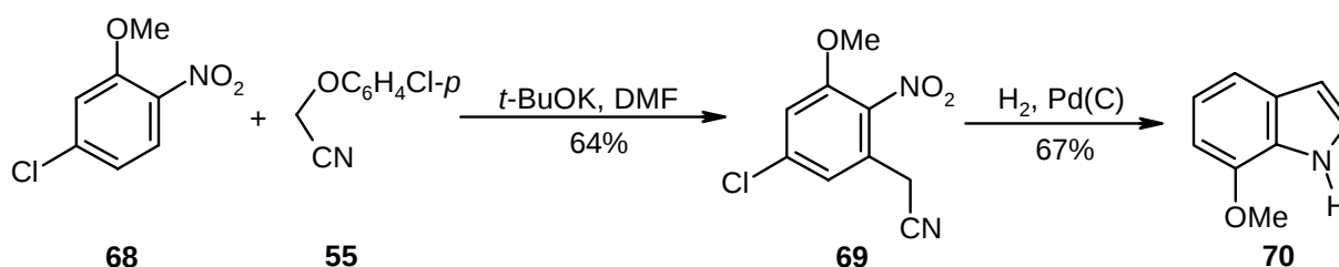
Scheme 19
