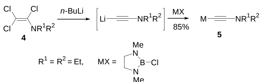
Trichloroenamines ( 4 ) can also undergo elimination to lithiated ynamines which can be trapped by halides to furnish hetero-substituted ynamines ( 5 ) (Scheme 3). 6
