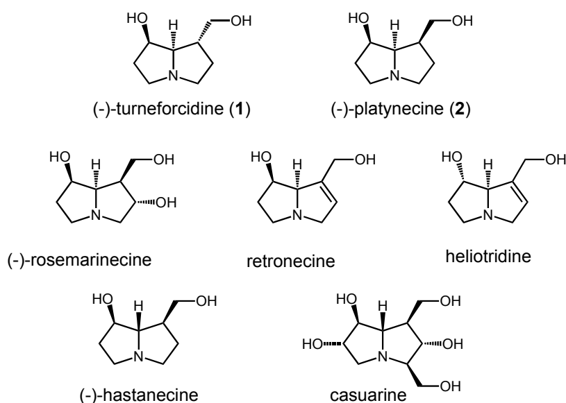
Figure 1. Representative pyrrolizidine alkaloids.
