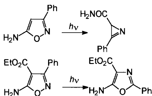
Scheme 6
