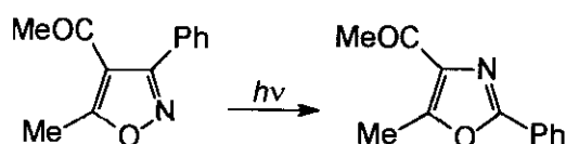
Scheme 8
