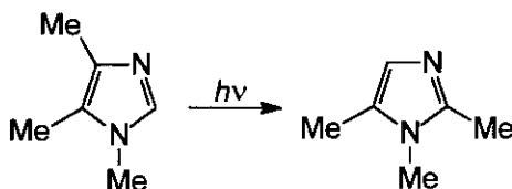
Scheme 12
