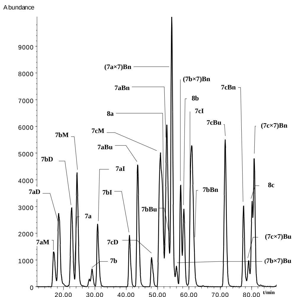
Figure 1: Total ion chromatogram of the library of amine additions to the enones ( 7a-c )
