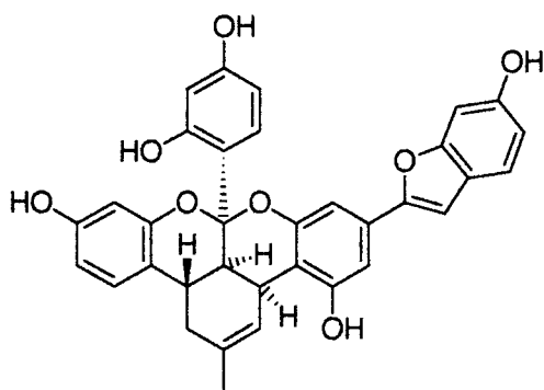
Figure 1. Structures of sanggenons C ( 1 ), D ( 2 ), O ( 13 ), mulberrofuran G ( 6 ), and their derivatives.
