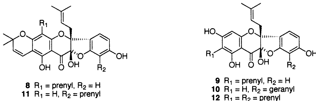
Figure 2. Structures of sanggenons L ( 8 ), sanggenols F ( 9 ), G ( 10 ), soroceins D ( 11 ), and F ( 12 ).
