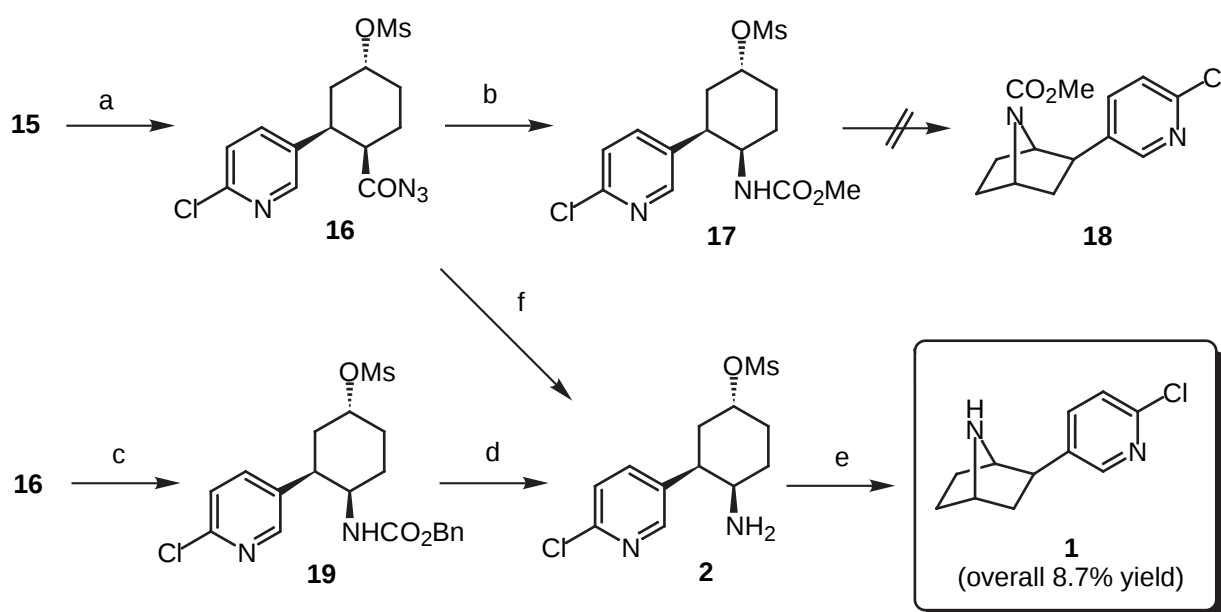
Scheme 3 a) MsCl, Et 3 N, acetone, 0°C., then NaN 3 , H 2 O. b) MeOH:C 6 H 6 (1:1), 70°C, 45% from 15 . c) BnOH, C 6 H 6 , 70°C, 77% from 15 . d) H 2 , 10%Pd/C, EtOH, HCl, 27%. e) CHCl 3 , reflux, quant. f) THF-H 2 O (2:1), conc. HCl (2 eq), reflux, 60% from 15 .
