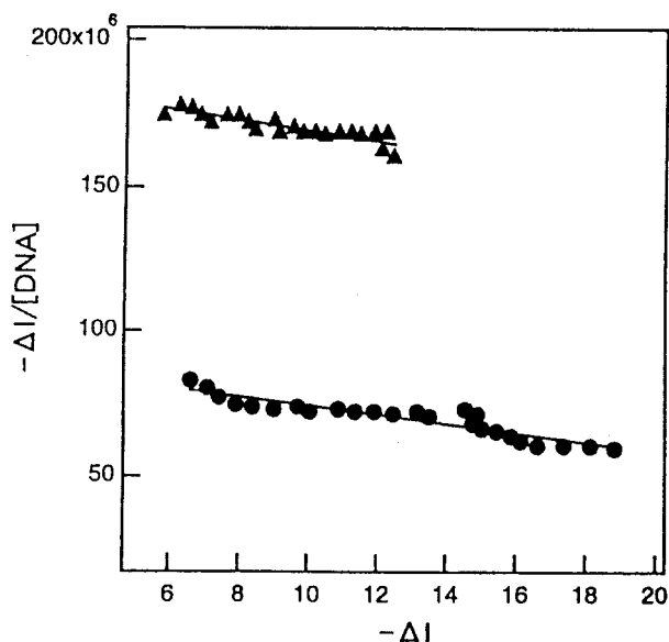
Figure 6 Scatchard plots of 8b -calf thymus DNA and 8b -12mer DNA ( 5'\text{-d(CATCCCGGGATG)-3'}_2 ) complexes. Fluorescence emission at 549.0 nm (excitation at 350.0 nm) of the complexes were used for the calculation; ●, calf thymus DNA; ▲, the 12mer DNA.
