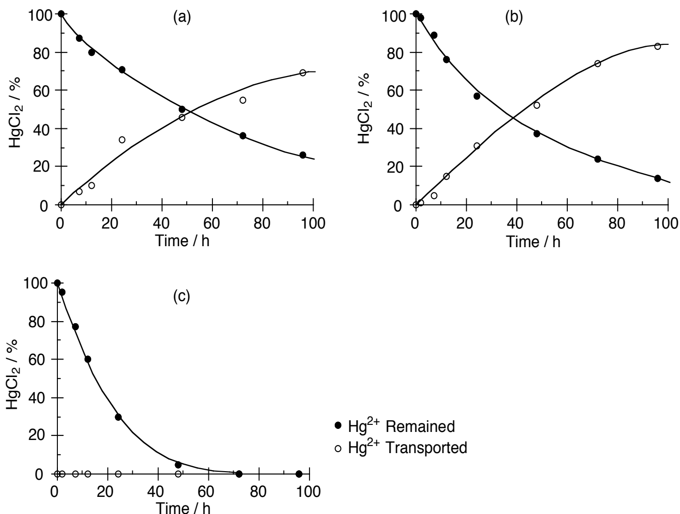
Figure 4. Transport of \text{Hg}^{2+} with (a) 4a , (b) 4b , and (c) 4c using 2 M HCl.
