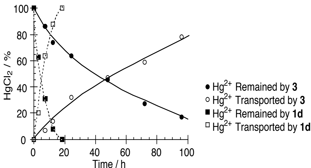
Figure 3. Transport of \text{Hg}^{2+} with 1d and 3 using 2 M HCl
