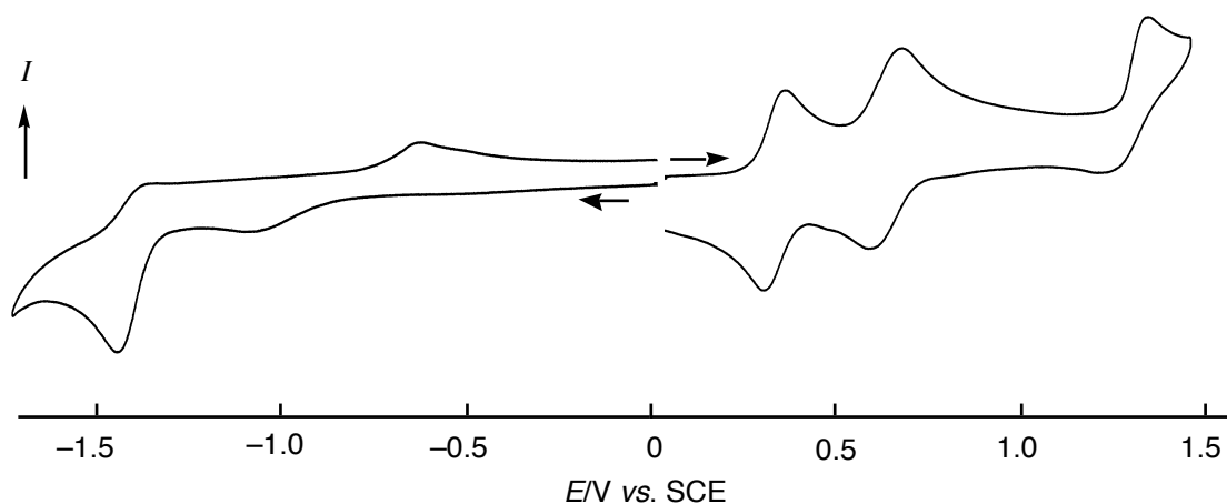
Figure 3. Cyclic voltammogram of 3d in 0.1 M Bu 4 NClO 4 /benzonitrile, scan rate = 100 mV/s.
