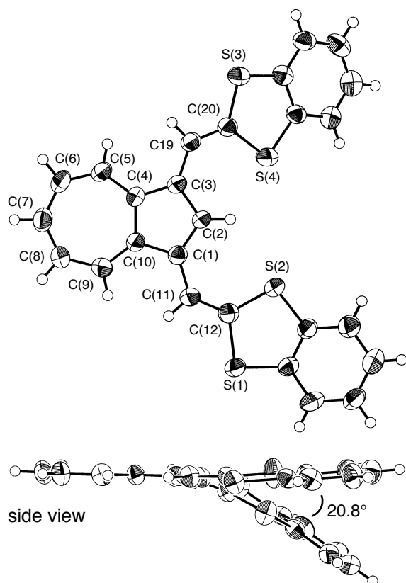
Figure 1. Molecular structure of 3d . Selected bond lengths ( \text{\AA} ): C(1)–C(2) 1.400(7); C(1)–C(10) 1.438(6); C(2)–C(3) 1.407(6); C(3)–C(4) 1.417(6); C(4)–C(5) 1.382(6); C(4)–C(10) 1.487(7); C(5)–C(6) 1.369(7); C(6)–C(7) 1.387(8); C(7)–C(8) 1.357(8); C(8)–C(9) 1.398(7); C(9)–C(10) 1.376(7).
