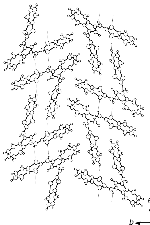
Figure 2. Crystal structure of 3d viewed along the c axis. Dotted lines indicate short S...H contacts ( < 3.0 \text{\AA} ).
