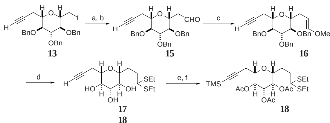
Scheme 3 Reagents and conditions. a) NaCN in DMSO. b) DIBAL-H, CH 2 Cl 2 (90 % in 2 steps). c) [Ph 3 PCH 2 OMe] + Cl - , t -BuLi (68 %). d) BF 3 •OEt 2 , EtSH, CH 2 Cl 2 . e) EtMgBr, TMSCl. f) Ac 2 O, Py, CH 2 Cl 2 (57 % in 3 steps).
