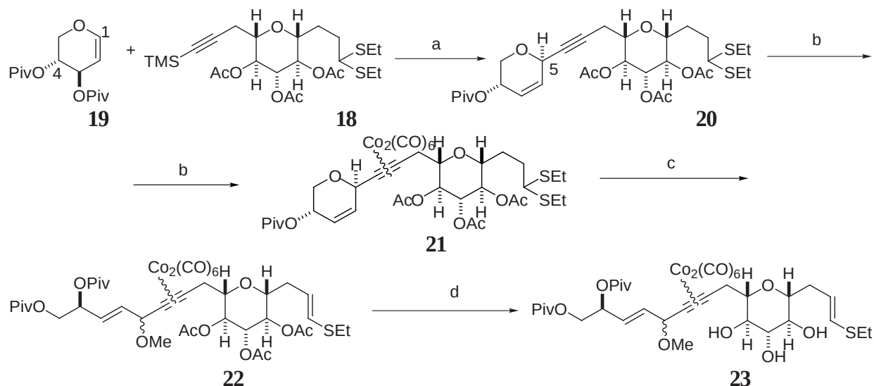
Scheme 4 Reagents and conditions. a) \text{SnCl}_4 in \text{CH}_2\text{Cl}_2 at -20^\circ\text{C} , 1 h (40 %). b) \text{Co}_2(\text{CO})_8 (97 %). c) \text{Piv}_2\text{O} , \text{TfOH} in \text{CH}_2\text{Cl}_2 then \text{MeOH} (73 %). d) \text{K}_2\text{CO}_3 , \text{MeOH} (98 %).
