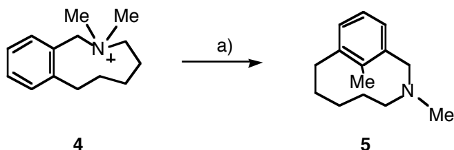
Scheme 1. a) \text{NaNH}_2/\text{NH}_3(l) .
