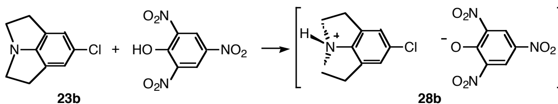
Scheme 9. \text{CDCl}_3 , rt
