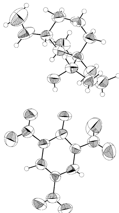
Figure 2. ORTEP drawing of the X-Ray structure of 22
