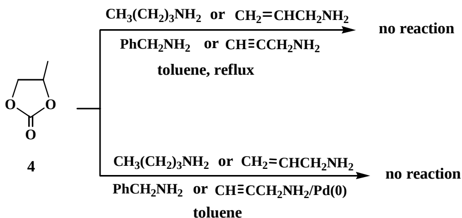
Scheme 9
