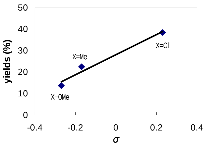
Figure 3. Hammett plot of Hammett's sigma values ( \sigma ) vs. yields of 4
