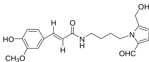
magnolamide ( 8 )
