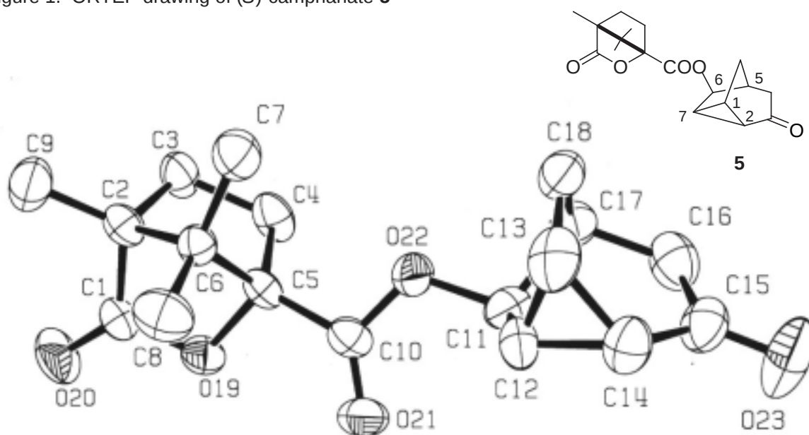
Figure 1. ORTEP drawing of ( S )-camphanate 5
