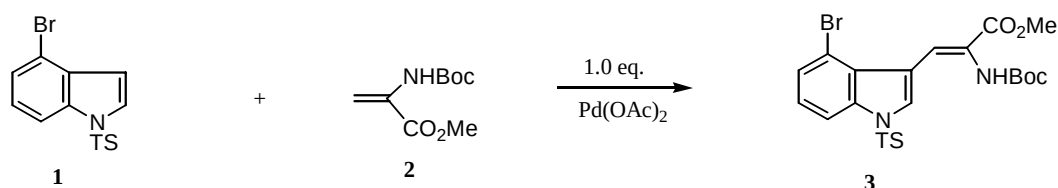
Scheme 1 : Direct C-3 Vinylation of 4-Bromo-1-tosylindole ( 1 ) for Synthesizing 4-Bromodehydrotryptophan Derivative ( 3 )
