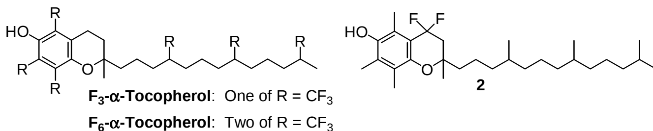
Figure 1. F 3 - or F 6 - \alpha -Tocopherols and 4,4-difluoro- \alpha -tocopherol ( 2 )
