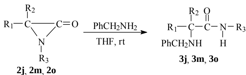
Scheme 9. The reaction of \alpha -lactams ( 2j , 2m , and 2o ) with benzylamine.
