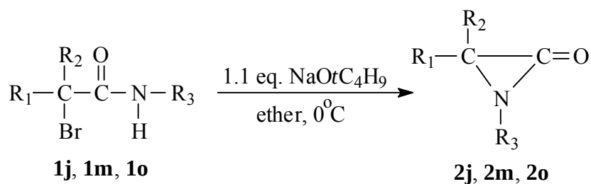
Scheme 8. Synthesis of \alpha -lactams ( 2j , 2m , 2o ).
