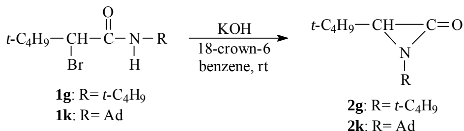
Scheme 7. The PTC synthesis of \alpha -lactams ( 2g and 2k ).
