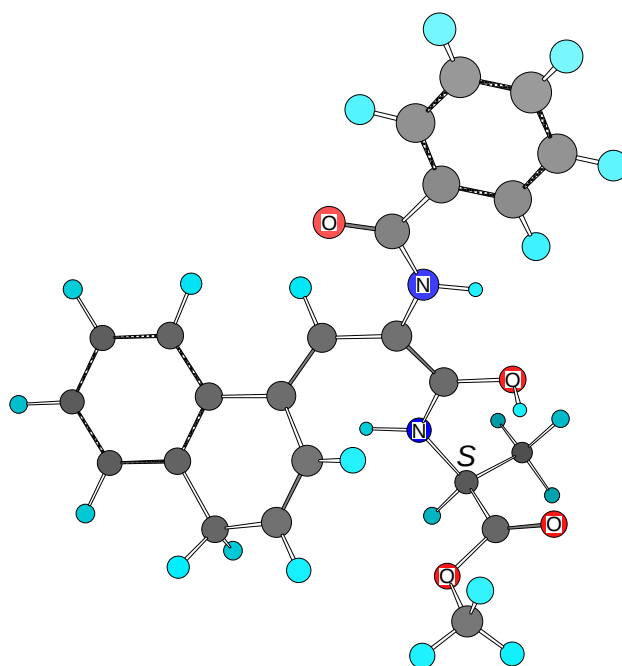
Figure 2. Energy-minimized conformation of II ( R' = Ph)
