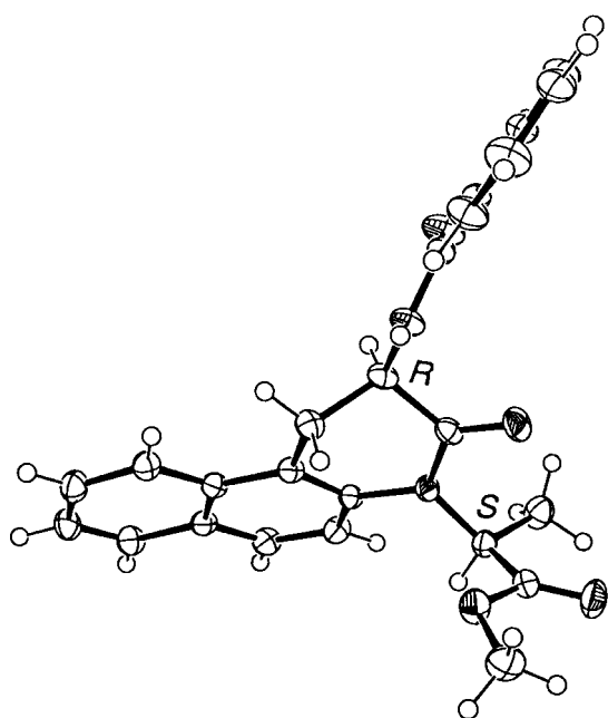
Figure 1. ORTEP drawing of ( R,S )- 2b
