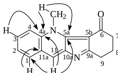
Figure 2 : Long range ^1\text{H} - ^{13}\text{C} NMR correlations of compound ( 21 ) observed from HMBC spectrum.
