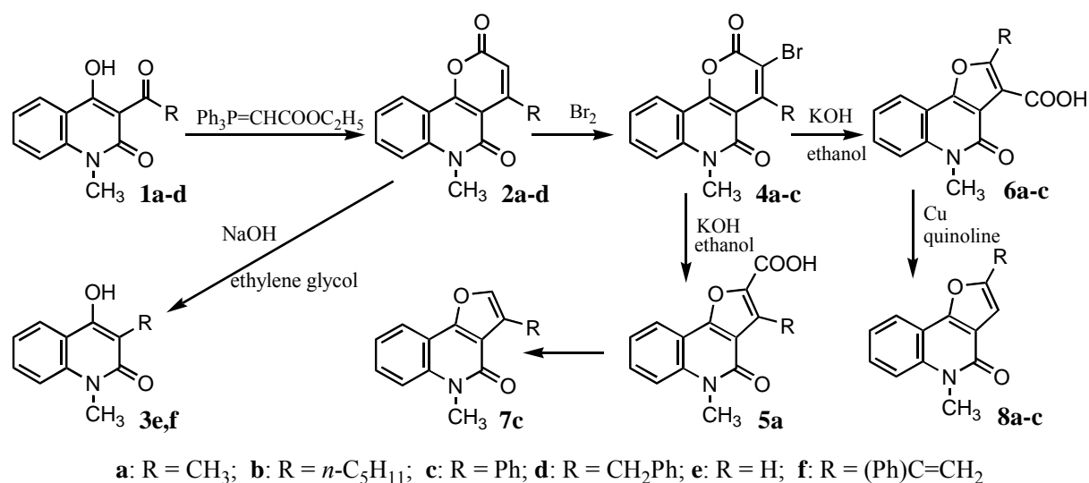
Scheme 1
