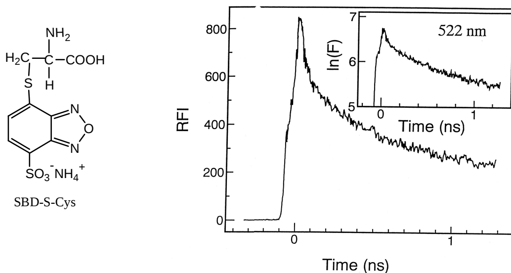
Figure 3. Time profile of fluorescence intensity of SBD-S-Cys in aqueous solution (pH 9). Insert: \ln(\text{fluorescence intensity}) vs. time.
