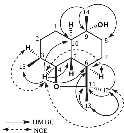
Figure 6. Important HMBC and NOESY correlations of 3 .
