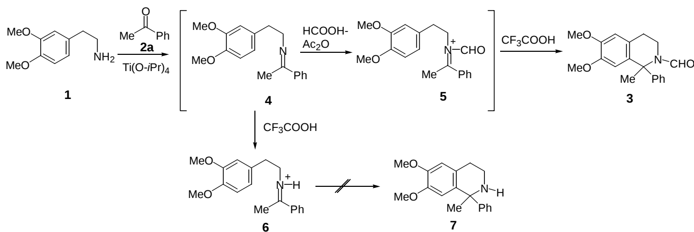
Scheme 1
