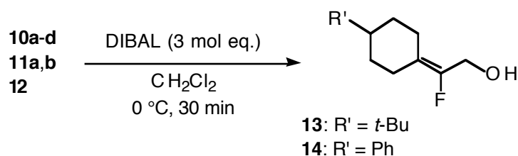
Scheme 5
