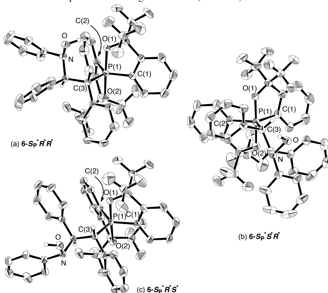
Figure 1. ORTEP drawings of (a) 6- \text{Sp}^*\text{R}^*\text{R}^* , (b) 6- \text{Sp}^*\text{S}^*\text{R}^* , and (c) 6- \text{Sp}^*\text{R}^*\text{S}^* showing the thermal ellipsoids at the 30% probability level.
