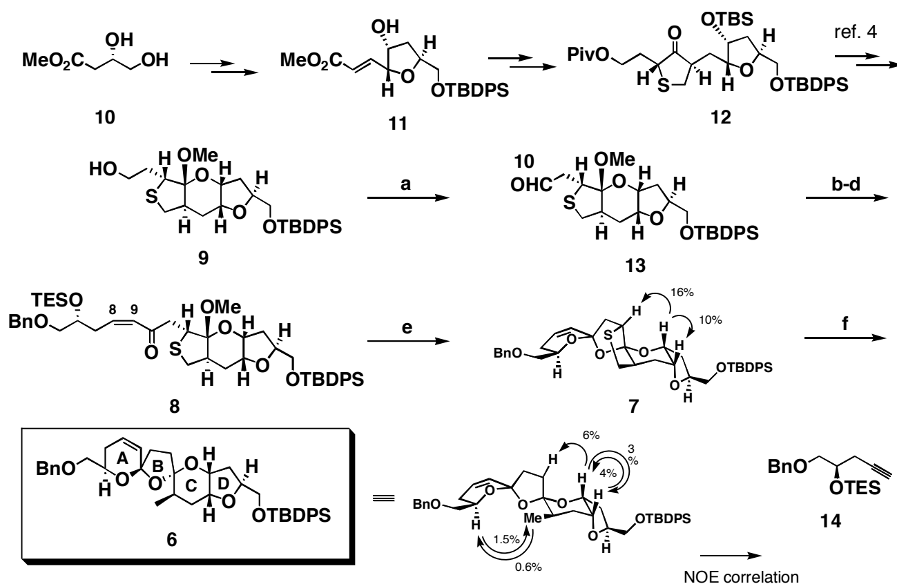
Scheme 2. Reagents and conditions: (a) \text{SO}_3\cdot\text{Py} , DMSO, \text{Et}_3\text{N} , \text{CH}_2\text{Cl}_2 , 90%; (b) 14 , n\text{-BuLi} , THF, -78^\circ\text{C} ; (c) \text{H}_2 , Lindlar cat., benzene; (d) \text{SO}_3\cdot\text{Py} , DMSO, i\text{-Pr}_2\text{NEt} , \text{CH}_2\text{Cl}_2 , 51% in 3 steps; (e) \text{Yb}(\text{OTf})_3 , MeCN, rt, 57%; (f) Raney Ni W-4, EtOH, reflux, 72%.
