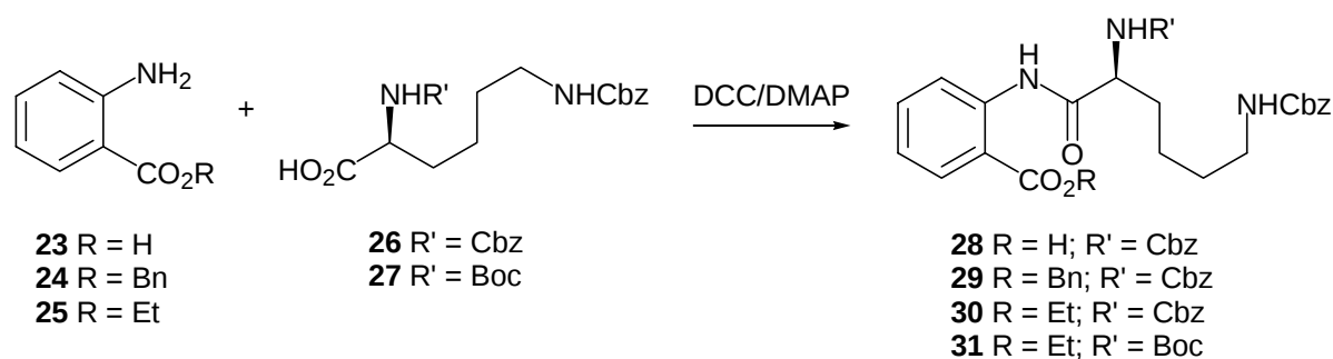
Scheme 4
