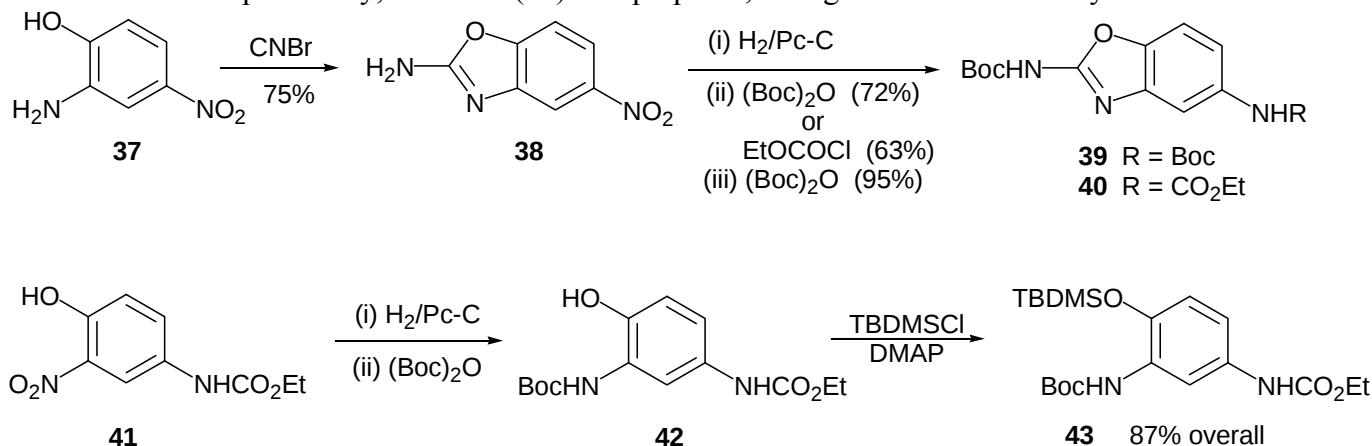
Scheme 5
