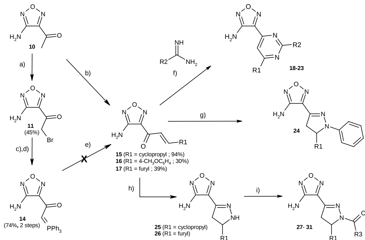
Scheme 4. a) Br 2 (1.05 eq.), AcOH (100%), 55°C; b) R 1 CHO (2.0 eq.), piperidine (0.1 eq.), C 2 H 5 OH /THF: 5/1, 50°C; c) PPh 3 (1.0 eq.), toluene, 100°C; d) NaOH (2N), CH 3 OH, 0°C; e) R 1 CHO (1.2 eq.), piperidine (0.1 eq.), 60°C; f) amidine or guanidine (1.1 eq.), N,N -dimethylacetamide, 60°C, O 2 (gas); g) PhNHNH 2 (2.0 eq.), THF/ C 2 H 5 OH: 1/20, rt; h) H 2 NNH 2 .H 2 O (10 eq.), THF, rt; i) R 3 COCl (1.2 eq.), pyridine (3.0 eq.), CH 2 Cl 2 , rt.
