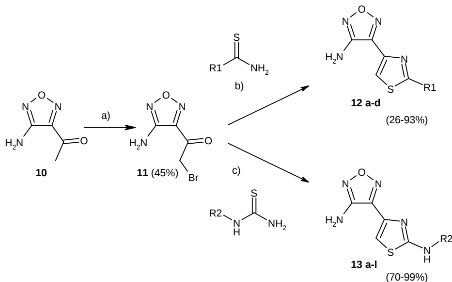
Scheme 3. a) Br 2 (1.05 eq.), AcOH (100%), 55°C; b) method A : 1.1 eq. nucleophile, benzene, reflux, 2-3 h, Dean-Stark; c) method B : 1.1 eq. nucleophile, C 2 H 5 OH, reflux, 2-3 h.
