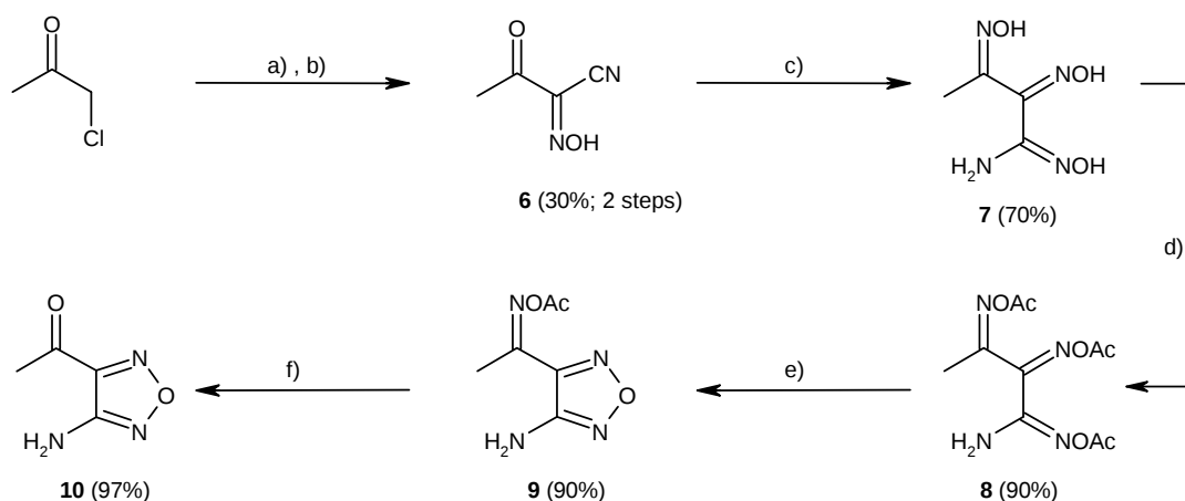
Scheme 2. a) isopentyl nitrite, (C 2 H 5 ) 2 O, HCl; b) KCN (1.8 eq.), (C 2 H 5 ) 2 O, H 2 O, 45°C ; c) H 2 NOH.HCl, NaOH, H 2 O, rt ; d) Ac 2 O, 0°C-rt ; e) NaOAc (4 eq.), dioxane, 60°C; f) 20% HCl, H 2 O, reflux, steam distillation.
