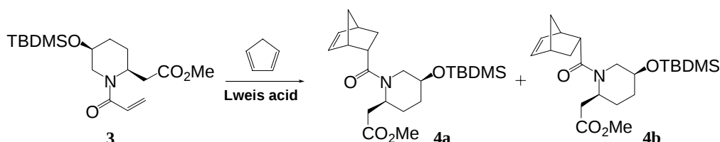
Scheme 1. Diels-Alder reaction of 3 with cyclopentadiene
