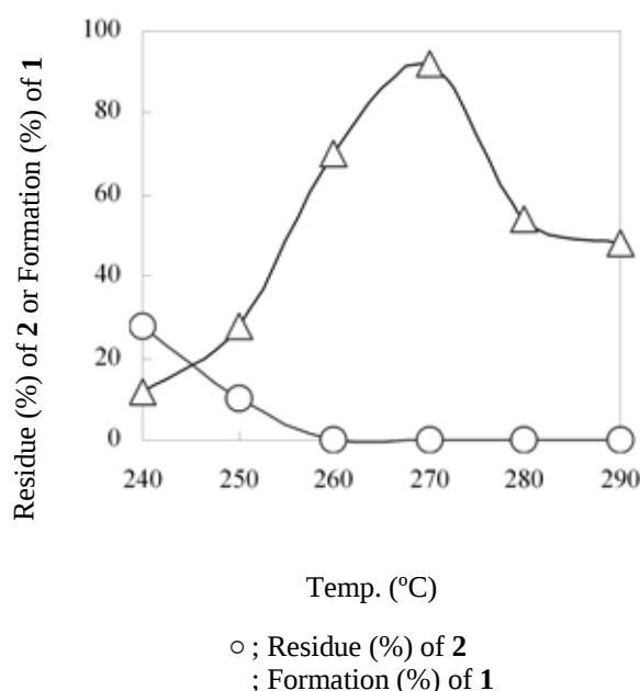
Figure 1. Hydrothermolysis of 2 and production of 1 .
