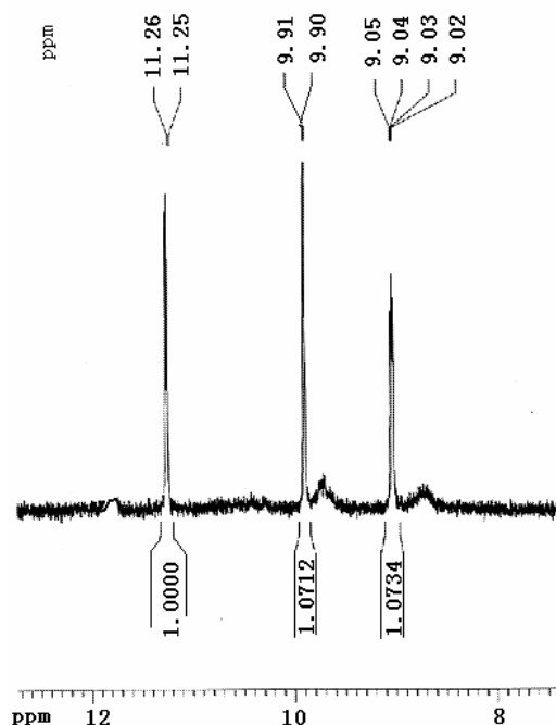
Figure 2. ^1\text{H} NMR (400 MHz, \text{CF}_3\text{COOD} ) spectra of azaPc( 1 )
