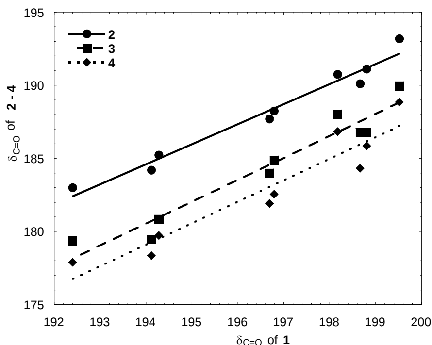
Figure 4. Plots of the \delta_{\text{C=O}} of 1a-c vs. \delta_{\text{C=O}} of 2-4 in all solvents. The slopes and correlation coefficients are: 2 , 1.371 (0.994); 3 , 1.496 (0.966); and 4 , 1.470 (0.948).
