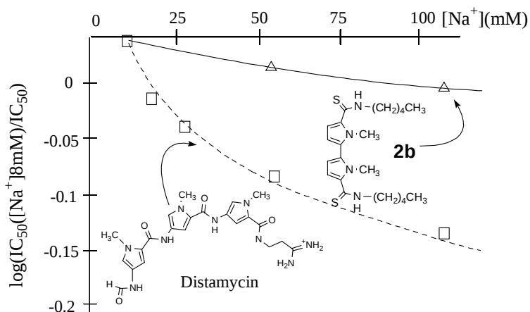
Figure 4. Comparison of Decrease of IC 50 Values Depending on NaCl Concentrations.
