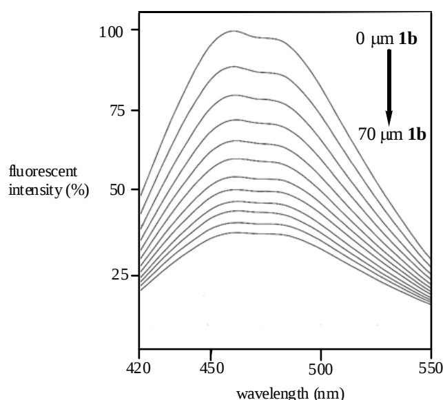
Figure 3. Change of Fluorescent Spectra in Displacement Assay of Hoechst 33258-CA12 with 1b . Emission spectra was obtained with \lambda_{\text{ex}} = 355 nm. See footnote of Table 1 for CA12.
