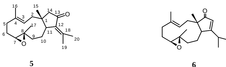
Figure 4 Structures of 5 and 6
